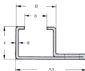
Profile 15
