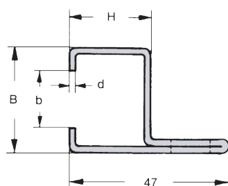
Profile 14
