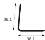
1.5° EXTERNAL ANGLE
