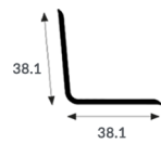
1.5° INTERNAL ANGLE *
