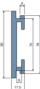
90mm side guide Part: MV-1057 Code: 105700BC-3m
