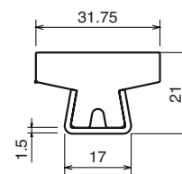
31.75mm T guide rail Part: MV-123 Code: 12301C-3m
