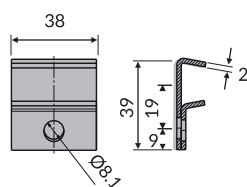
Single clamp Part: MV-328 Code: 32801
