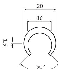
16mm round bar cover Part: MV-166 Code: 16604-30m
