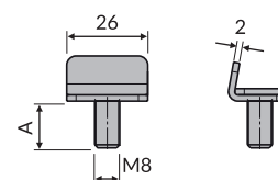
Single clamp M8 Part: MV-330 Code: 33001 a=15 Code: 33002 a=26 Code: 33003 a=20
