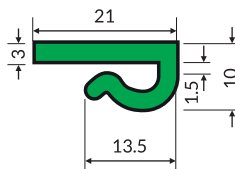
Z-clip profile without nose Part: MV-103 Code: 10302-60m Fits on: 2.5m up to 3.5m
