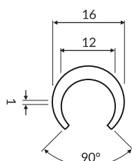
12mm round bar cover Part: MV-166 Code: 16603-30m
