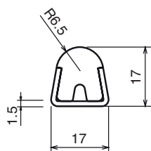
Round guide rail Part: MV-119 Code: 11901C-3m
