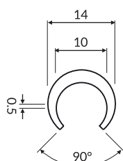
10mm round bar cover Part: MV-166 Code: 16602-30m
