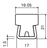
19.05mm T guide rail Part: MV-143 Code: 14301C-3m
