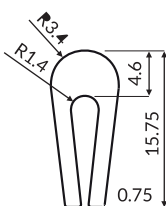
1.5mm snap on Part: MV-1001 Code: 100103-30m
