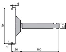
Stainless steel clamps Part: MV-331 Code: 33102 a=12 Code: 33103 a=16
