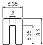
1.5mm snap on Part: MV-1000 Code: 100003-30m
