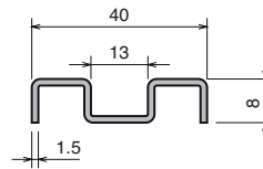
Stainless steel profile Part: MV-117 Code: 11701C-3m
