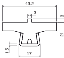
43.2mm T guide rail Part: MV-142 Code: 14201C-3m
