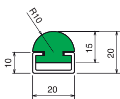
Standard guide rail Part: MV-134 Code: 13401C-3m
