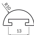
20mm round profile
