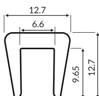
6mm snap on Part: MV-1009 Code: 100903-30m
