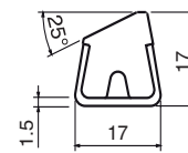
25° guide rail Part: MV-152 Code: 15201C-3m
