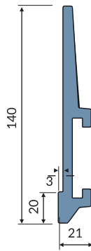
140mm side guide Part: MV-189 Code: 18900BC-3m
