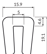
4mm/5mm snap on Part: MV-153 Code: 15303-30m
