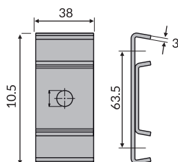
Double clamp Part: MV-329 Code: 32901
