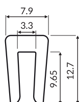
3mm snap on Part: MV-1004 Code: 100403-30m
