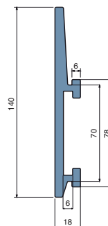
140mm side guide Part: MV-193 Code: 19320BC-3m
