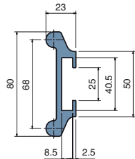
80mm side guide Part: MV-183 Code: 18301BC-3m
