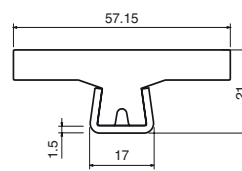
57.15mm T guide rail Part: MV-141 Code: 14101C-3m
