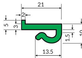
Z-clip profile with nose Part: MV-104 Code: 10402-60m Fits on: 2.5m up to 3.5m
