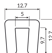
5mm snap on Part: MV-1006 Code: 100603-30m
