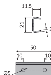
Connecting bar Part: MV-390 Code: 39001
