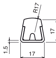
Modified guide rail Part: MV-120 Code: 12001C-3m
