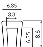
3mm snap on Part: MV-1002 Code: 100203-30m
