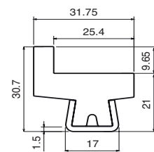
31.75mm L guide rail Part: MV-144 Code: 14401C-3m
