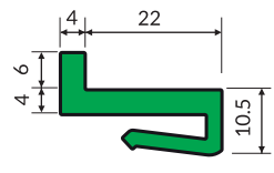
Z-clip profile with nose Part: MV-179 Code: 17902C-3m Fits on: 2.5m up to 3.5m
