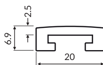
20mm curved profile
