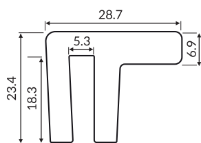
5mm snap on Part: MV-1008 Code: 100803C-3m
