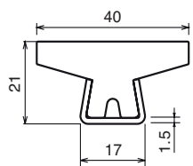
40mm T guide rail Part: MV-124 Code: 12401C-3m
