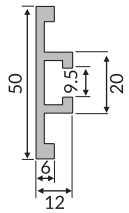
Aluminium profile Part: MV-159 Code: 15901C-3m
