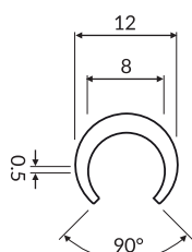
8mm round bar cover Part: MV-166 Code: 16601-30m
