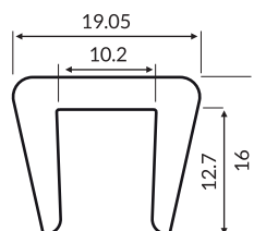
10mm snap on Part: MV-1011 Code: 101103-30m
