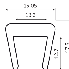
12mm/13mm snap on Part: MV-1012 Code: 101203-30m
