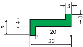
Z profile reinforced Part: MV-102 Code: 10202-60m
