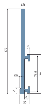
170mm side guide Part: MV-187 Code: 18730BC-3m
