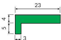
L profile Part: MV-175 Code: 17502-60m
