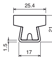
25.4mm T guide rail Part: MV-122 Code: 12201C-3m
