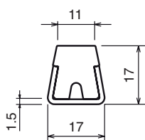
Flat guide rail Part: MV-121 Code: 12101C-3m
